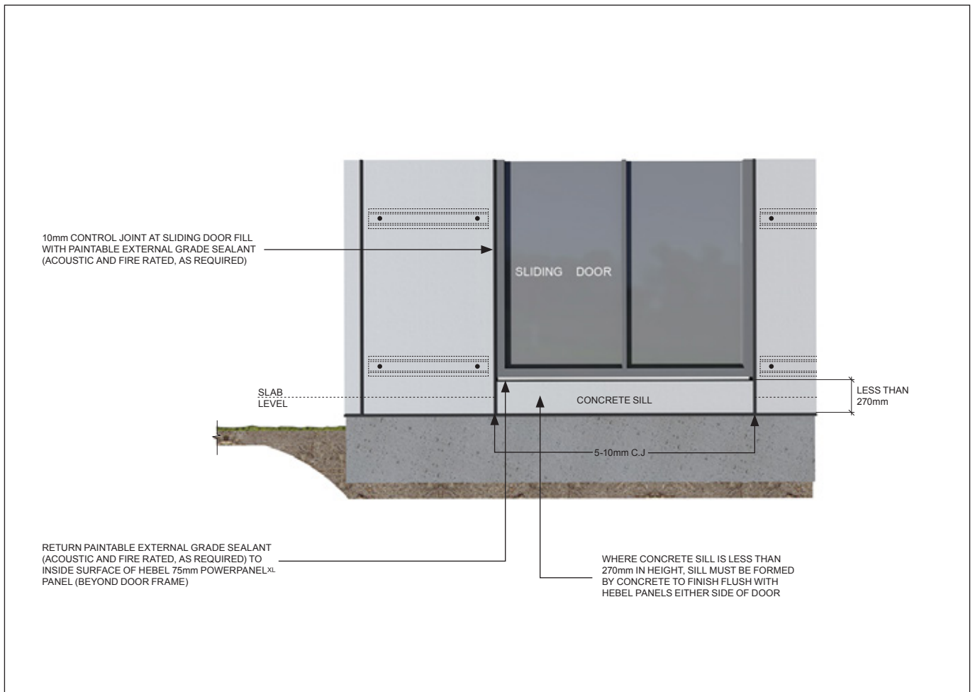
Detail 3.52 – Sliding door sill detail – option 1 – concrete sill < 270mm
