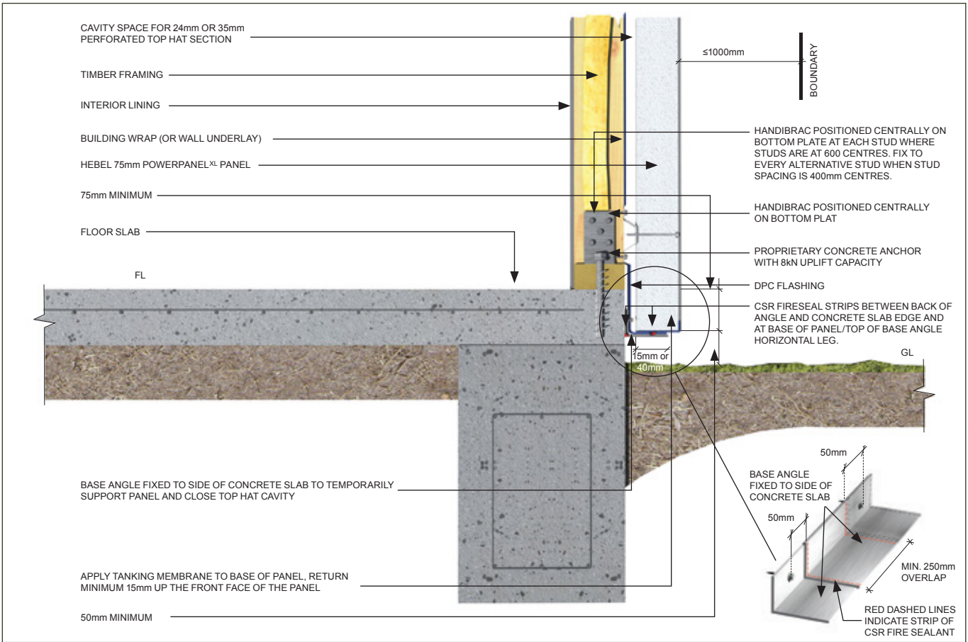
Fig. 2.1– 75mm PowerPanel XL Boundary Wall - Suspended Panel Base Detail
