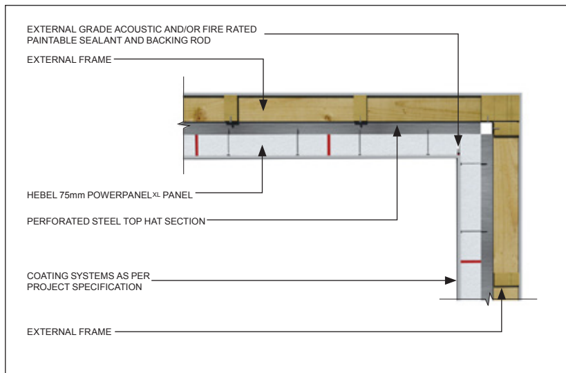
Detail 3.34 – Internal corner
