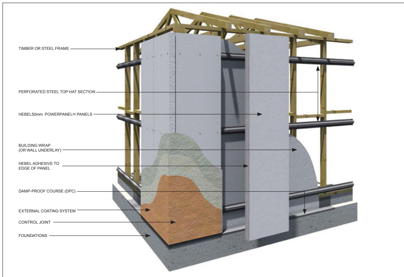
Fig. 1.1 – Typical Home Construction Application
