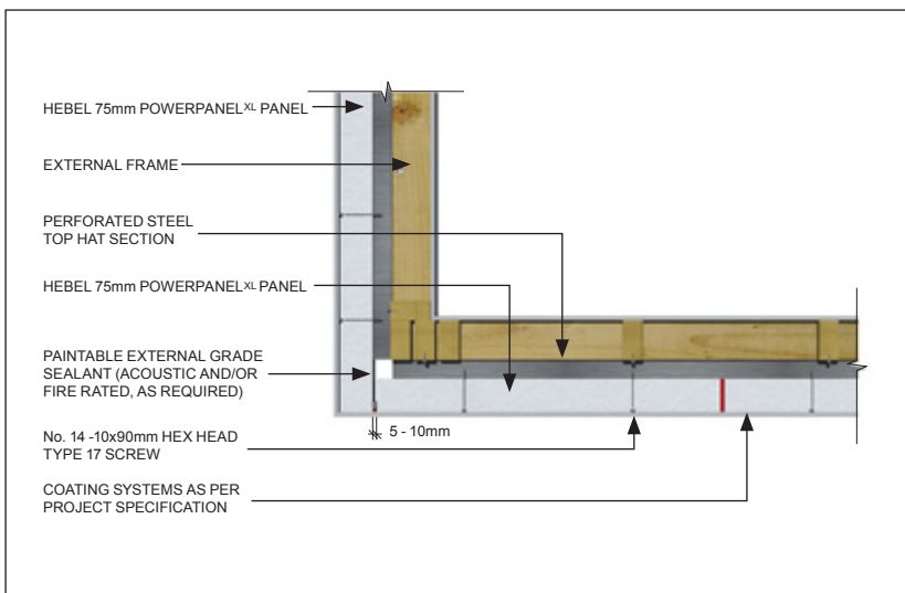
Detail 3.35 – External corner
