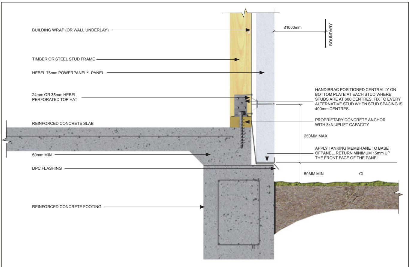
Fig. 2.2– 75mm PowerPanel XL Boundary Wall - Slab Supported Panel Base Detail
