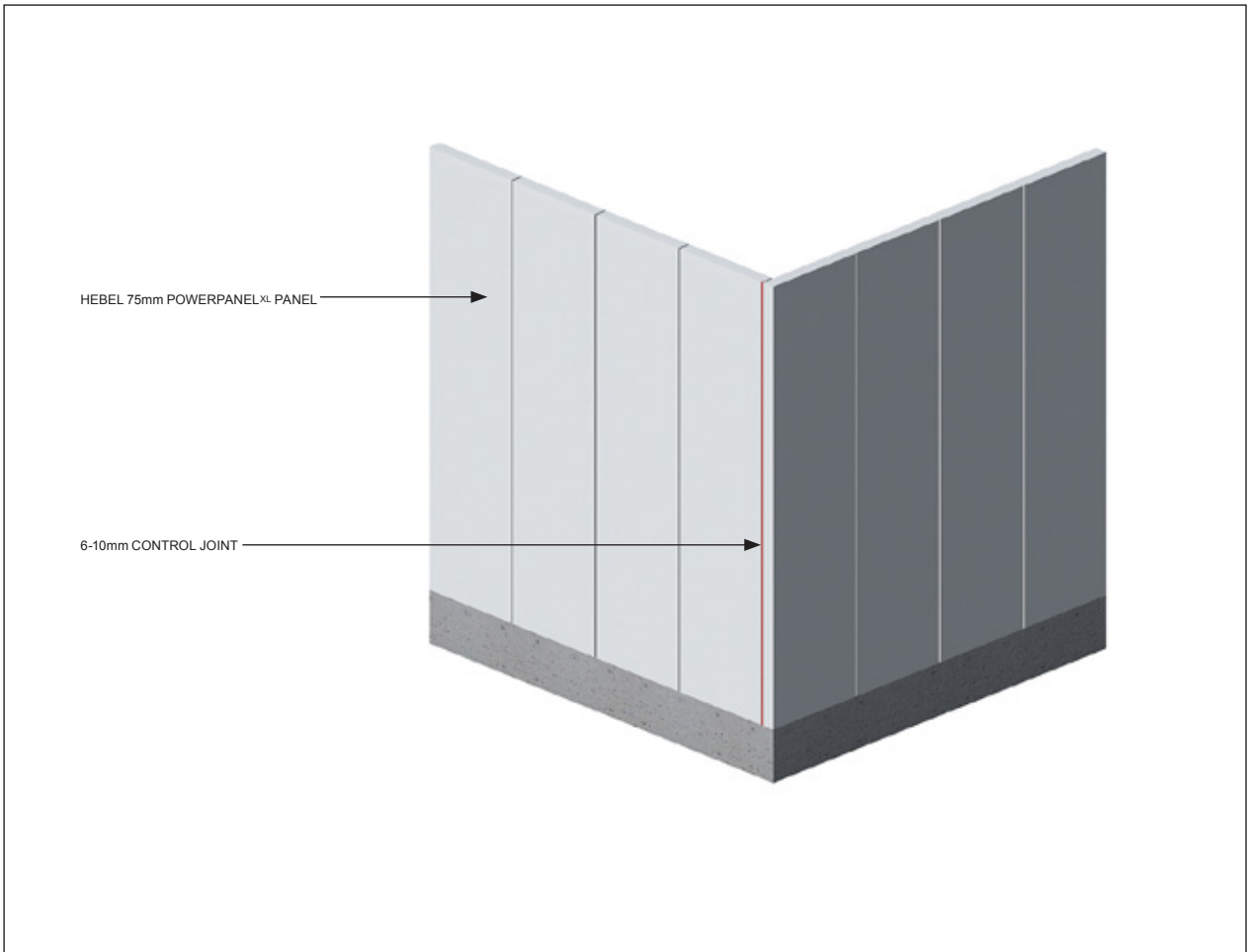
Detail 3.37 – Typical detail for control joints positioned on corner
