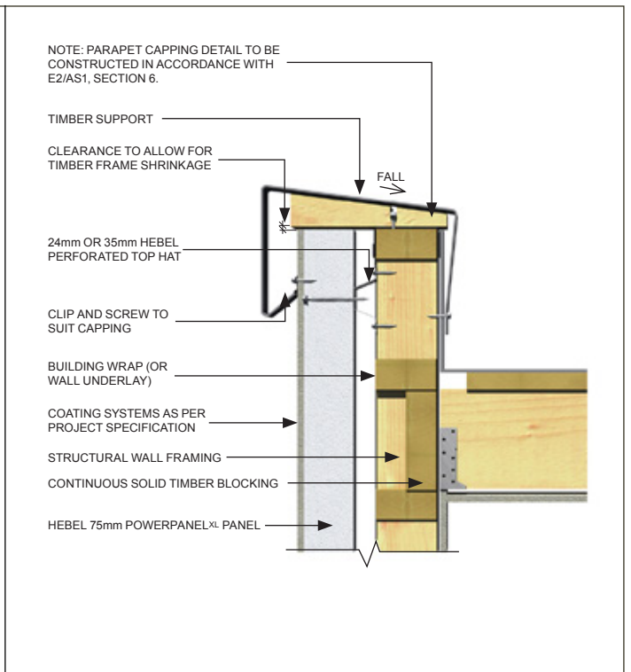
Fig. 2.5- 75mm PowerPanel XL Boundary Wall - Parapet Detail
