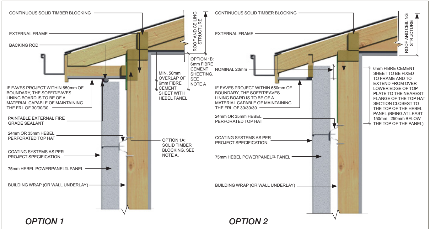
Fig. 2.3- 75mm PowerPanel XL Boundary Wall - Typical Eaves Detail
